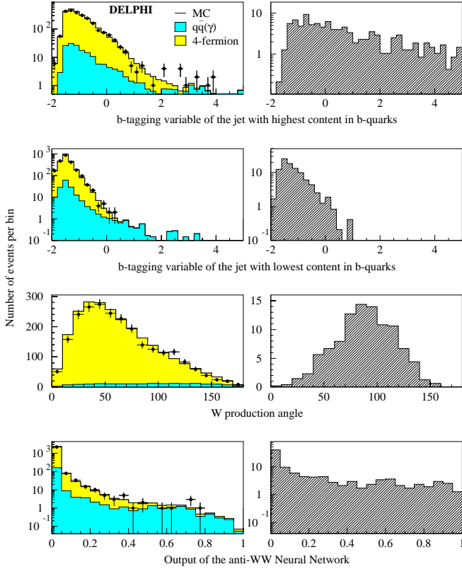
Fig. 7. Search in the semileptonic final state: distributions after the rejection of non-WW background. The plots on the left show the data (points) and the expected SM backgrounds (histograms) for the full DELPHI statistics at \sqrt{s} = 192 - 208 GeV. Those on the right show the technicolor signal in e^+e^- \rightarrow W\pi_T expected if M_{\pi_T} = 100 GeV. The signal normalisation corresponds to M_{\rho_T} = 220 GeV/ c^2 , N_D = 9 and the integrated luminosity collected at \sqrt{s}=192\text{--}208 GeV
