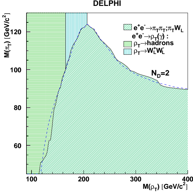
Fig. 9. The region in the (M_{\rho_T} - M_{\pi_T}) plane (filled area) excluded at 95% CL for N_D = 2 (maximal W_L - \pi_T mixing). The dashed line shows the expected limit for the e^+e^- \rightarrow \pi_T \pi_T, \pi_T W_L search
