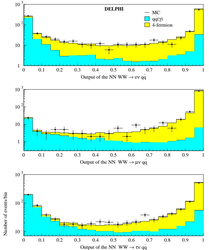
Fig. 6. Search in the semileptonic final state: neural network outputs for the rejection of non-WW backgrounds for events with an electron candidate (top), a muon candidate (centre), or a tau candidate (bottom)
