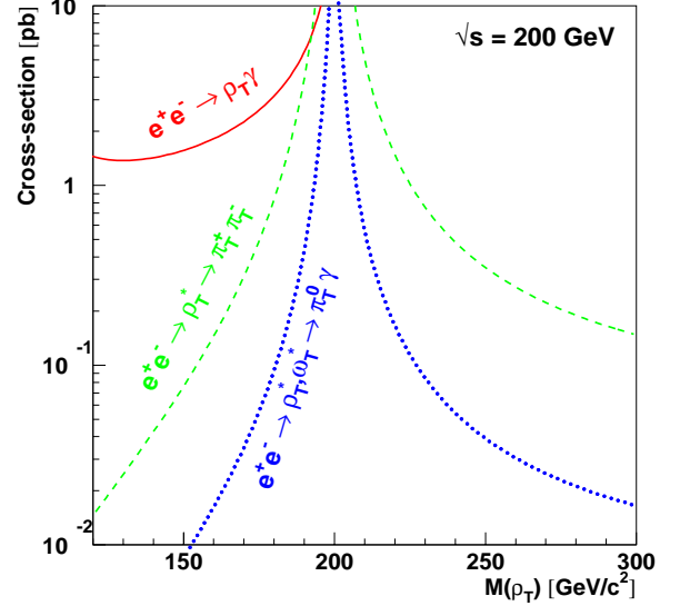
Fig. 1. Technicolor production cross-sections at LEP for some typical parameter values: M_{\pi_T} = 90 GeV/c 2 , M_V = 200 GeV/c 2 , N_D = 9 , (Q_U + Q_D) = 4/3 , and \alpha_{\rho_T} = 2.91(3/N_{TC}) with N_{TC} = 4
