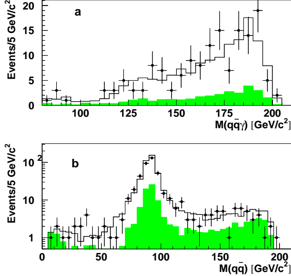
Fig. 11a,b. \pi_T^0\gamma analysis: a distribution of the mass of the hadronic system plus the isolated photon; b distribution of the hadronic mass. The points show the data, the histogram shows the contribution of standard sources, and the filled histogram shows separately the contribution of all non- b\bar{b}\gamma processes. The statistics shown in a and b ) corresponds to different event selections, see the text for details
