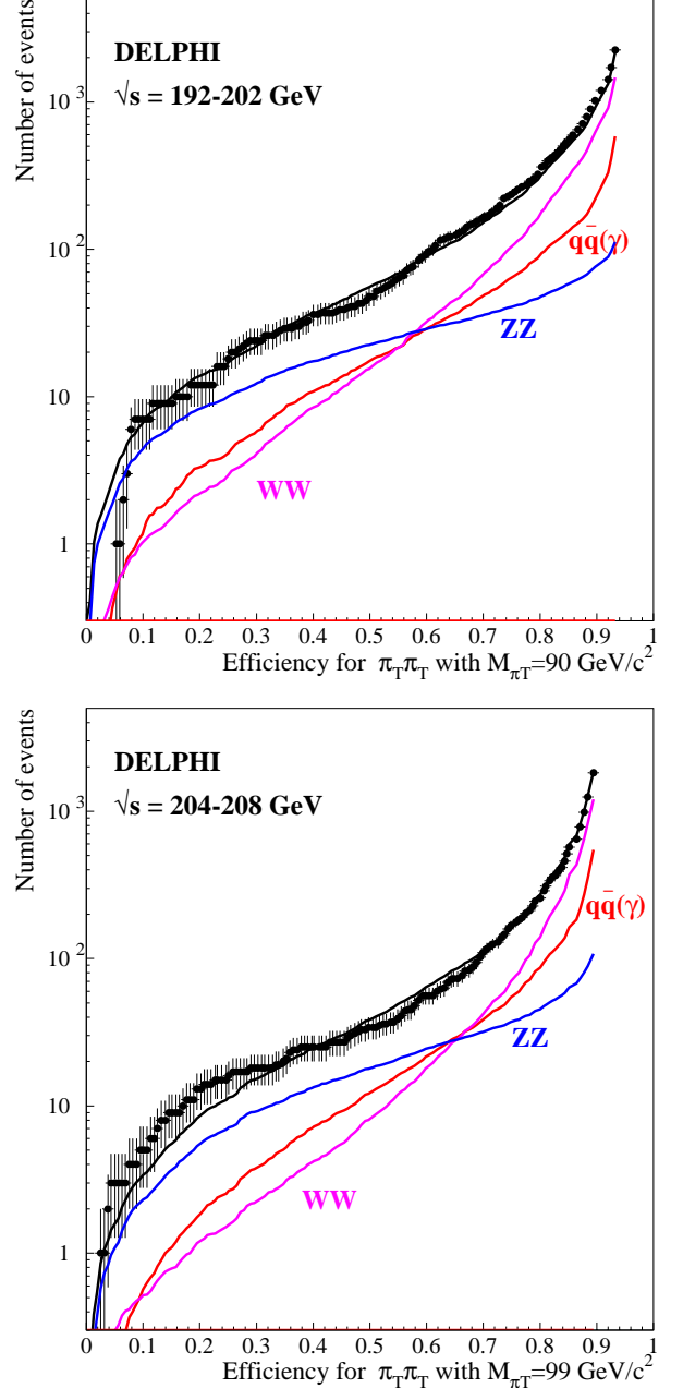
Fig. 4. Search in the 4-jet final state: numbers of data events (points) and expected SM background events (curves) as a function of the \pi_T\pi_T signal efficiency, varied by varying the cut on the neural network variable. The different background contributions are shown both separately and combined. The two plots show the two different years of data taking considered
