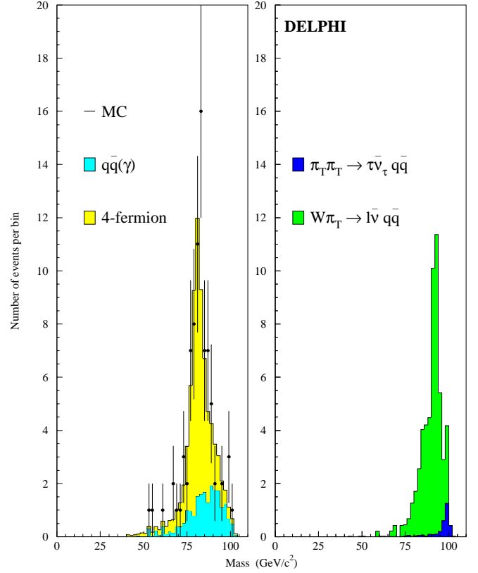
Fig. 8. Search in the semileptonic final state: Estimated \pi_T mass distributions for NN output > 0.10. The plot on the left shows the data (points) and the expected SM backgrounds (histograms) for the full DELPHI statistics at \sqrt{s} = 192 - 208 GeV. The one on the right shows the technicolor signals in e^+e^- \rightarrow \pi_T\pi_T and e^+e^- \rightarrow W_L\pi_T expected if M_{\pi_T} = 100 GeV/ c^2 , M_{\rho_T} = 220 GeV/ c^2 and N_D = 9 , normalised to the integrated luminosity collected at \sqrt{s} = 192 - 208 GeV
