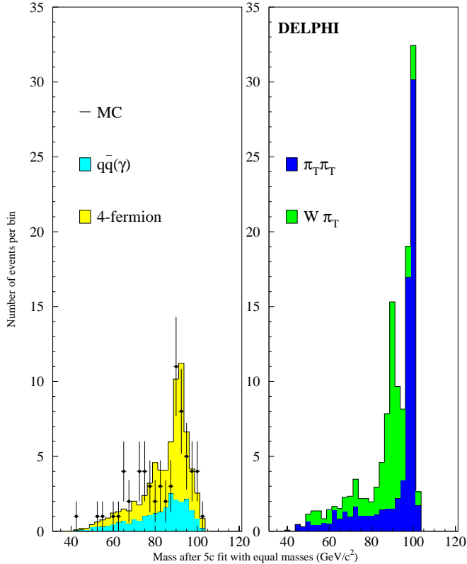
Fig. 5. Search in the 4-jet final state: M_{5C} mass distributions for the NN analysis with the cut on NN output > 0.30 . The plot on the left shows the data (points) and the expected SM backgrounds (histograms) for the full DELPHI statistics at \sqrt{s} = 192 - 208 GeV. The one on the right shows the technicolor signals in e^+e^- \rightarrow \pi_T\pi_T and e^+e^- \rightarrow W_L\pi_T expected if M_{\pi_T} = 99 GeV/ c^2 , M_{\rho_T} = 220 GeV/ c^2 and N_D = 9 , normalised to the integrated luminosity collected at \sqrt{s} = 192 - 208 GeV
