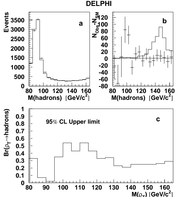
Fig. 13. a Mass distribution of the hadronic system in the e^+e^- \rightarrow q\bar{q}(\gamma) analysis for the data collected at \sqrt{s} = 183 and 189 GeV. Crosses show the data and the histogram shows the SM contribution. b Difference between the observed numbers of events and those expected in the SM. The expected contribution of \rho_T \rightarrow \pi_T\pi_T with M_{\rho_T} = 150 GeV/c 2 and M_{\pi_T} = 70 GeV/c 2 is shown as the histogram. c The 95% CL upper limit on the branching ratio BR(\rho_T \rightarrow \text{hadrons})
