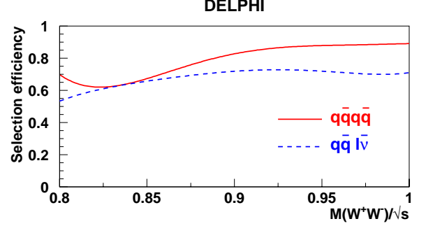
Fig. 12. Selection efficiency of a WW -like final state as a function of M(W^+W^-)/\sqrt{s} for \sqrt{s} = 206 GeV
