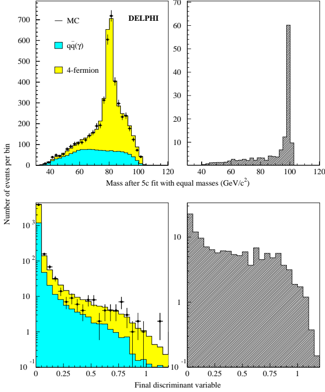
Fig. 3. Search in the 4-jet final state: distributions of the mass and final discriminant variable after preselection. The plots on the left show the data (points) and the expected SM backgrounds (histograms) for the full DELPHI statistics at \sqrt{s} = 192 - 208 GeV. Those on the right show the technicolor signal in e^+e^- \rightarrow \pi_T\pi_T expected if M_{\pi_T} = 99 GeV/ c^2 . The signal normalisation corresponds to M_{\rho_T} = 220 GeV/ c^2 , N_D = 9 and the integrated luminosity collected at \sqrt{s}=192-208 GeV
