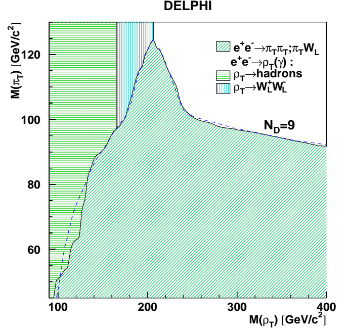
Fig. 10. The region in the (M_{\rho_T} - M_{\pi_T}) plane (filled area) excluded at 95% CL for N_D = 9 (theoretically preferred W_L - \pi_T mixing). The dashed line shows the expected limit for the e^+e^- \rightarrow \pi_T \pi_T, \pi_T W_L search
