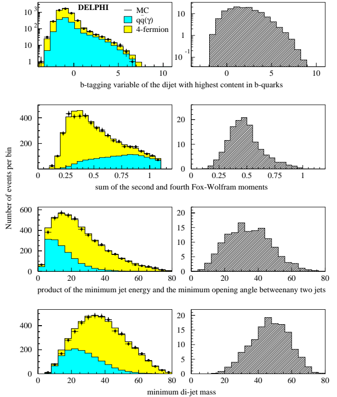
Fig. 2. Search in the 4-jet final state: distributions after preselection of the b -tagging variable, H_2 + H_4 , the product of the minimum jet energy and the minimum opening angle between any two jets. The plots on the left show the data (points) and the expected SM backgrounds (histograms) for the full DELPHI statistics at \sqrt{s} = 192 - 208 GeV. Those on the right show the technicolor signal expected in the channel e^+e^- \rightarrow \pi_T\pi_T if M_{\pi_T} = 99 GeV/ c^2 . The signal normalisation corresponds to M_{\rho_T} = 220 GeV/ c^2 , N_D = 9 and the integrated luminosity collected at \sqrt{s}=192-208 GeV
